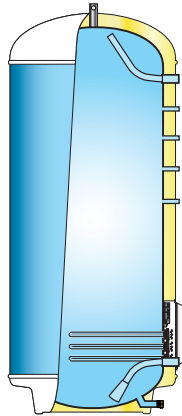
Electric heating of DHW in larger systems. 15 kW immersion. 300 - 1000 litre
