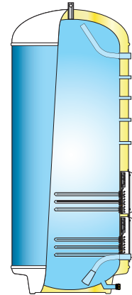
Electric heating of DHW in larger systems. 30kW immersion 400 - 1000 litre
