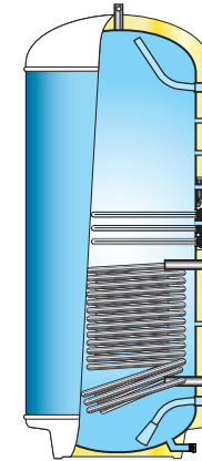
Designed especially for indirect heating with geothermal heat pump. 2.6 - 4.6m 2 coils. Electric backup 15 kW. 400 - 1000 litre
