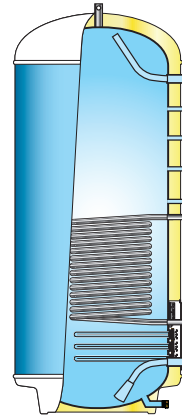
Cylinder with 1,00m 2 stainless steel coil for indirect heating from external heat source. Electric backup available 15kW. 400 - 1000 litre
